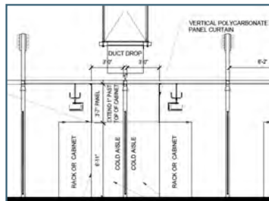
SPS Containment Drawing
