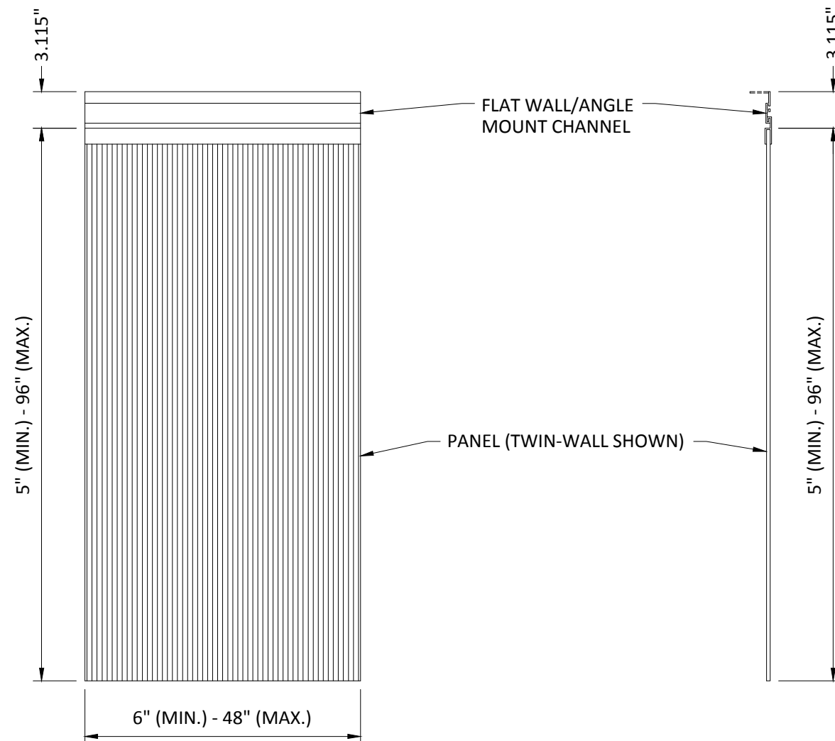
FRONT VIEW
