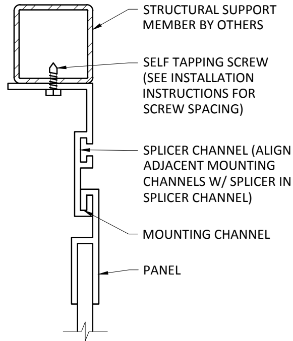
ANGLE MOUNT TO STRUCTURAL SUPPORT MEMBER MOUNTING DETAIL
