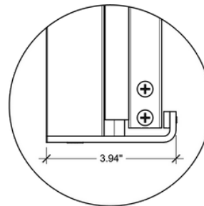
SIDE FOOTPAD DETAIL
