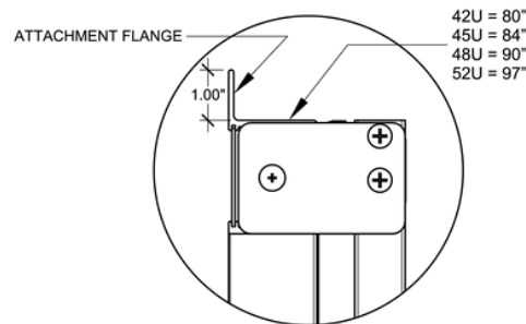
SIDE TOP DETAIL
