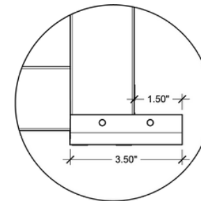
FRONT FOOTPAD DETAIL
