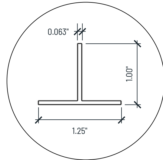
LITE TEE CROSS SECTION DIMENSIONS
