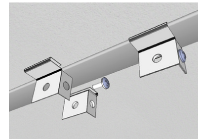
P-Clip Attaches to T-Bar
