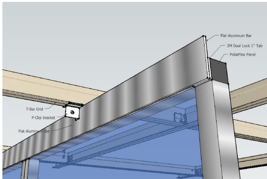
Panel Attached to Ceiling
